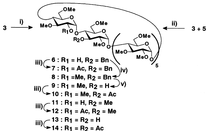
Scheme 2. Reagents and conditions: (i) LAH, \text{AlCl}_3 , THF, 0°C→rt; (ii) 80% aq. AcOH, 90°C; (iii) \text{Ac}_2\text{O} , pyridine; (iv) NaH, MeI, THF, rt; (v) \text{H}_2 , \text{Pd}(\text{OH})_2 , MeOH, rt.
