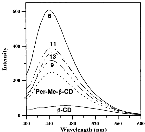
Figure 1. The fluorescence emission spectra excited at 366 nm of TNS at 20°C.
